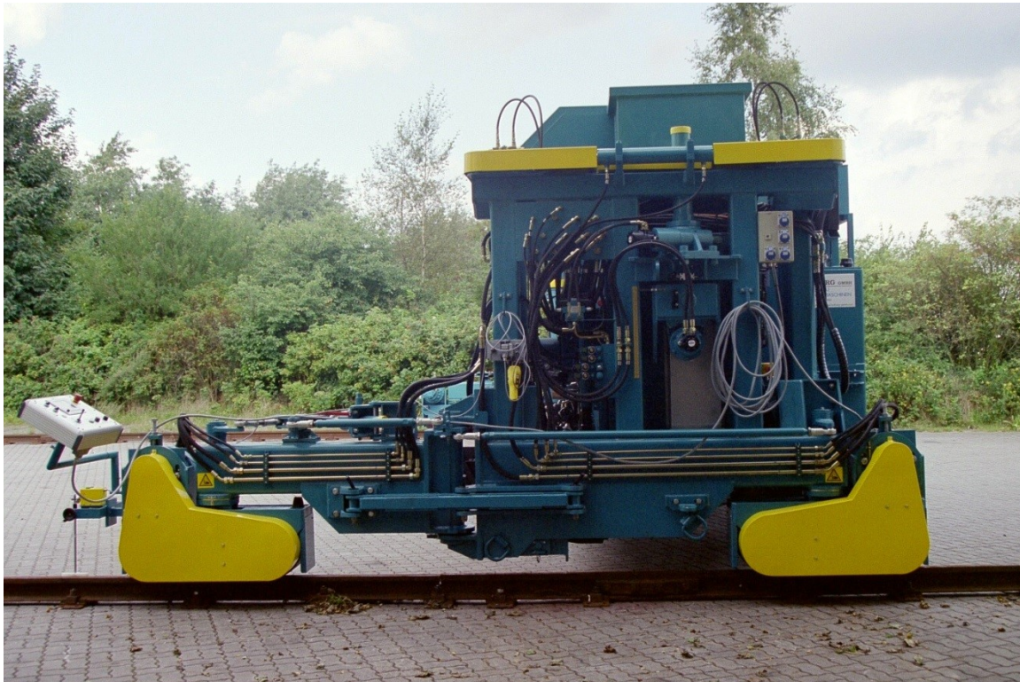
finisher KBR 140 side bulkhead with steerable front drive
